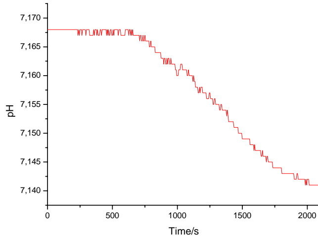
Figure 13: pH-time profile for 19.5 cm distance of sensor from the signal generation
