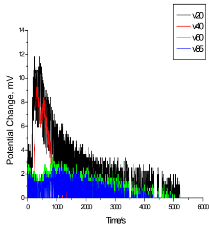
Figure 7: Change in the signal in the four sensors following the addition of 0.2 ml HCl 1M
