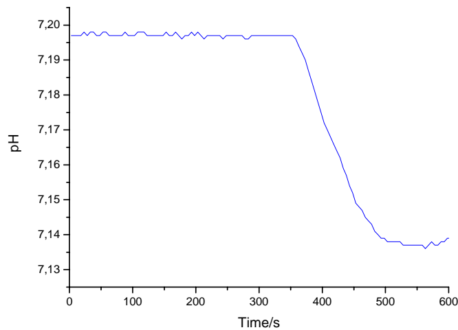
Figure 14: pH-time profile for 6.5 cm distance of sensor from the signal generation
