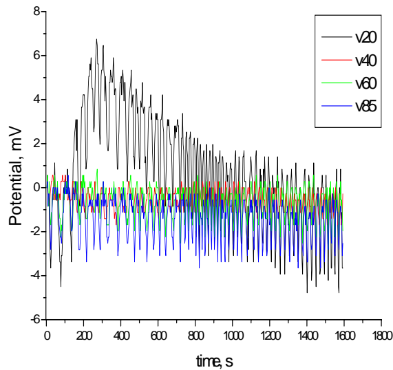
Figure 6: Change in the signal in the four sensors following the addition of 0.02 ml HCl 1M
