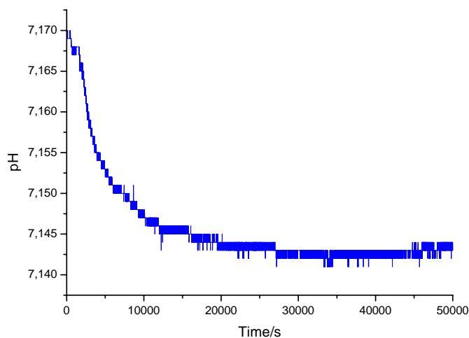
Figure 12: pH-time profile for 29.5 cm distance of sensor from the signal generation
