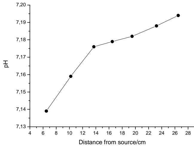
Figure 17: Dependence of the signal on the position of the sensor from the source of signal generation (readings taken 2000s past the acid spike on the top of the static fluid).
