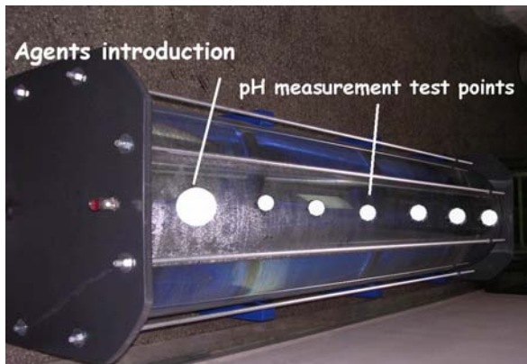
Figure 5: Ports on the simulator for the introduction of the agents and of pH sensors
