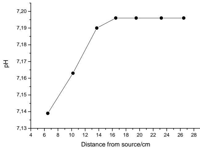
Figure 16: Dependence of the signal on the position of the sensor from the source of signal generation (readings taken 1000 s past the acid spike on the top of the static fluid).
