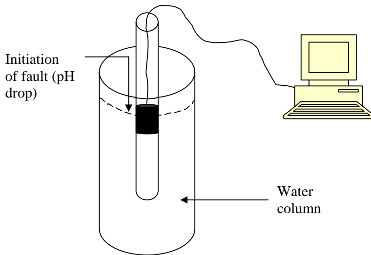
Figure 2: Experimental set-up for recording pH at different immersion depths with respect to the fault initiation ( H^+ ion release)
