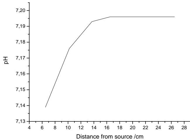
Figure 15: Dependence of the signal on the position of the sensor from the source of signal generation (readings taken 500 s past the acid spike on the top of the static fluid).
